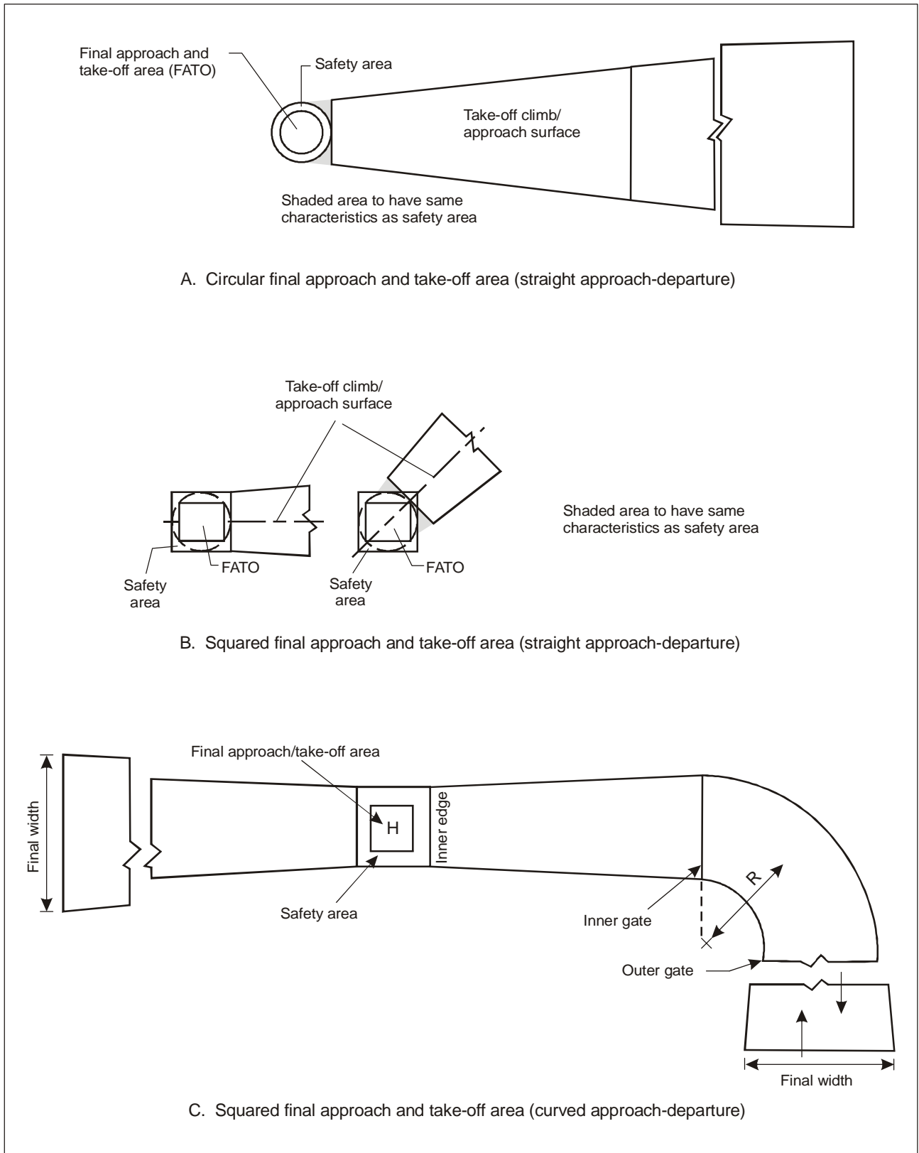
Figure 4-4. Take-off climb/approach surface (non-instrument FATO)
