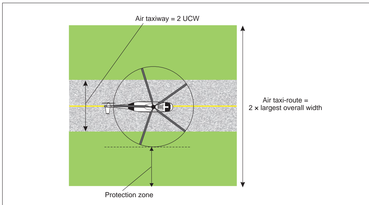
Figure 3-3. Air taxi-route
